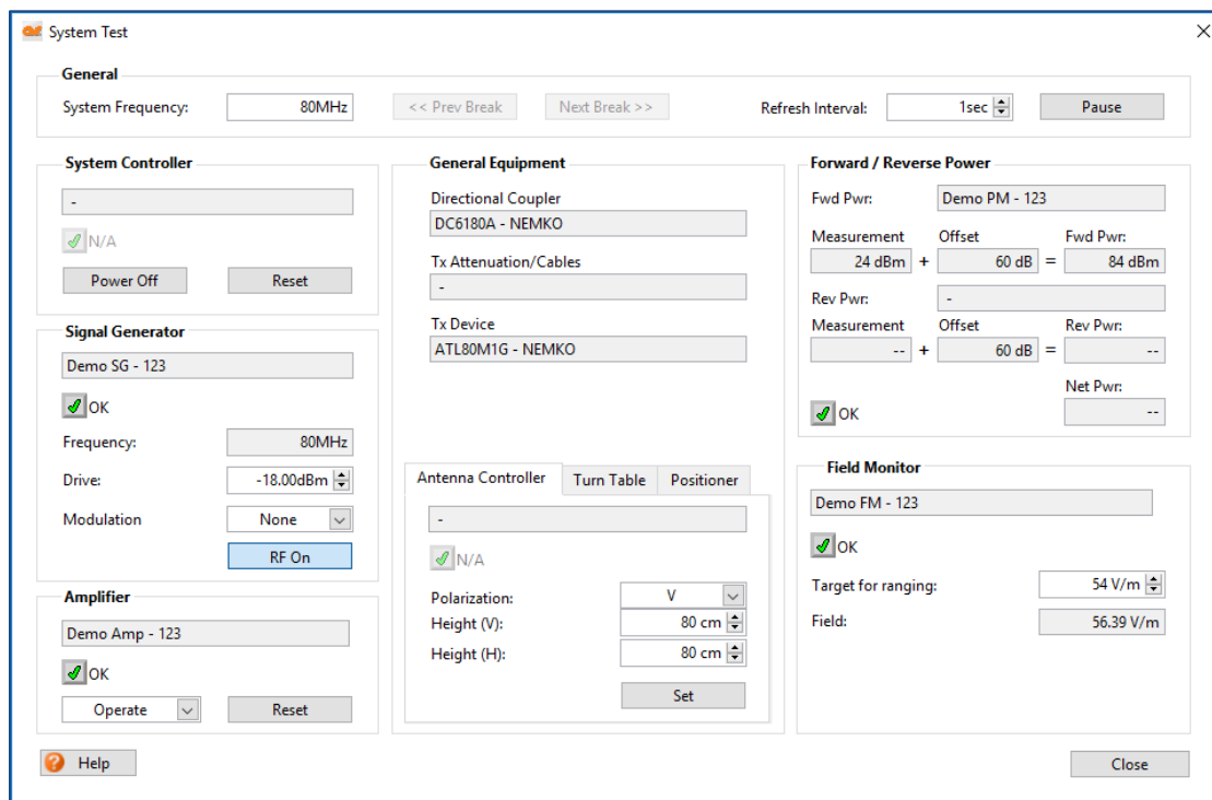
Figure 7 – System Test
