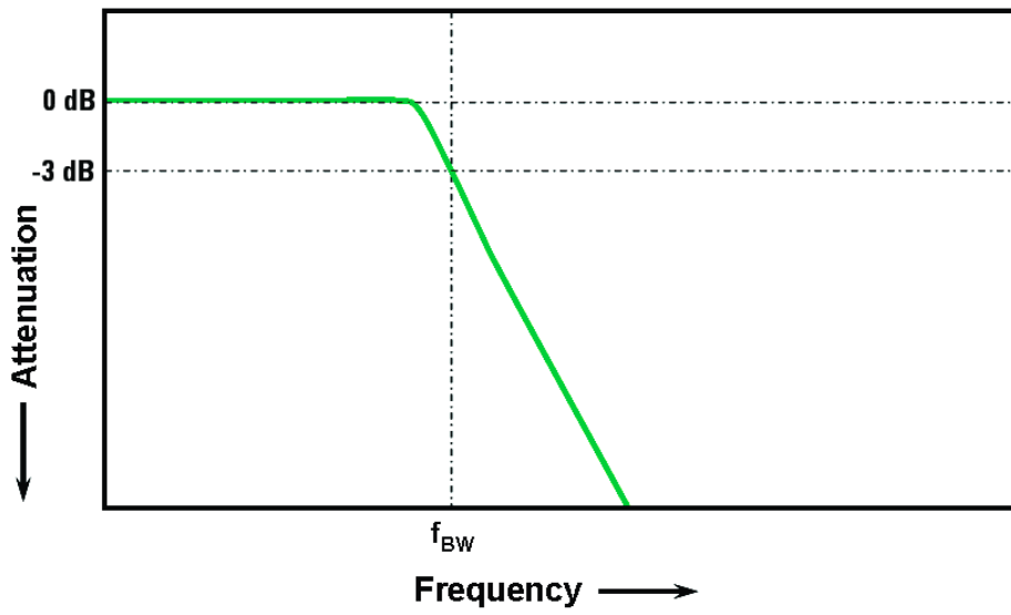
Figure 2. Oscilloscope maximally-flat frequency response
