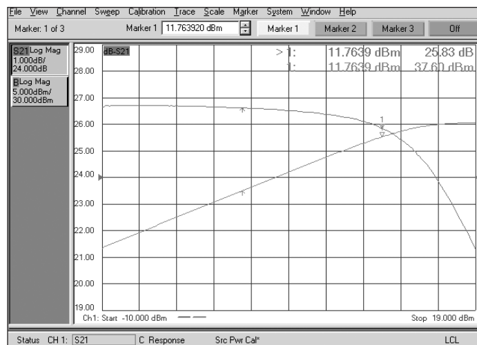
Figure 12. Amplifier gain compression
