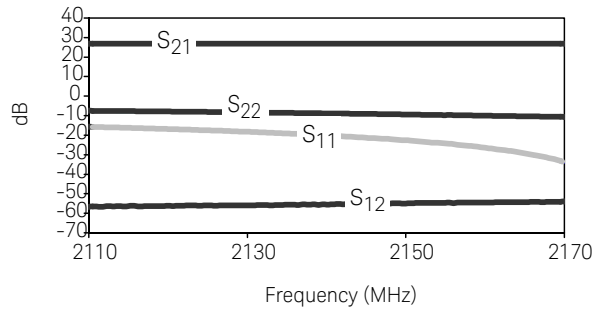
Figure 9. DUT S-parameters, with and without pre-amplifier
