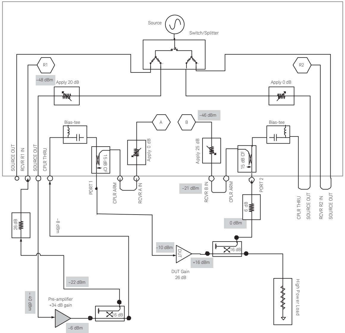
Figure 8. High-power setup, for low-power testing of S-parameters
