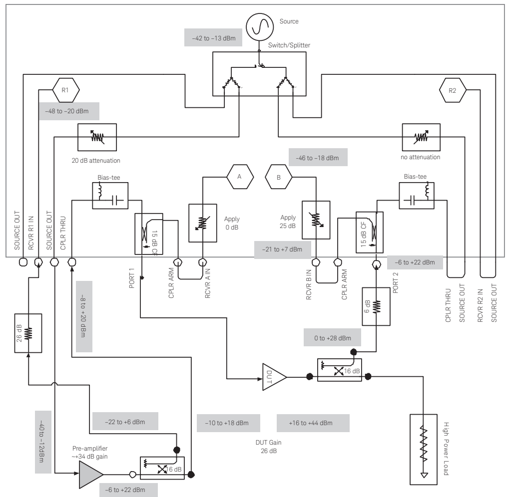
Figure 11. A power sweep for gain compression test.
