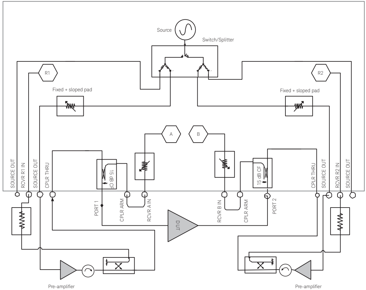
Figure 14. Two-way high-power measurements
