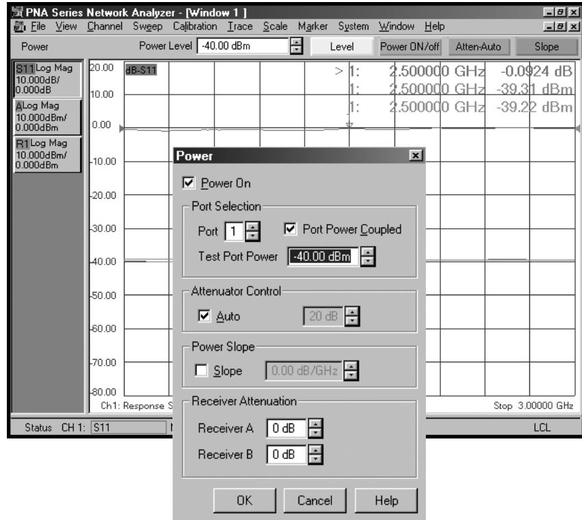
Figure 2. Case A, -40 dBm power level, 20 dB source attenuator
