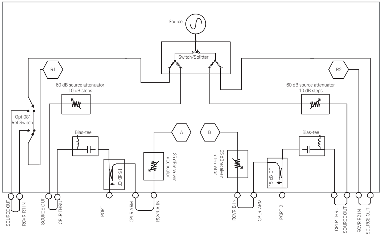
Figure 1. PNA (E8362/3/4B) block diagram for basic measurements
