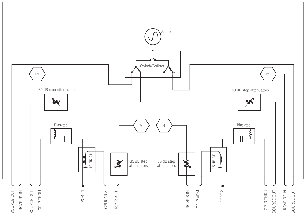
Figure 1. MW PNA E8362B block diagram, configured with source attenuators, receiver attenuators, bias-tees, and frequency-offset mode. (Options 016, UNL, 014, 080)
