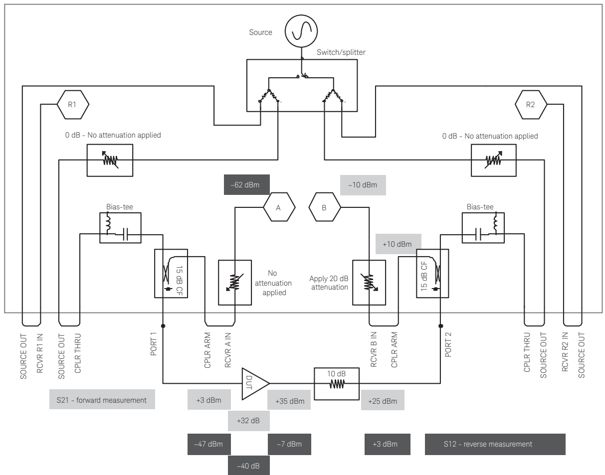
Figure 2. MW PNA E8362B, configured to measure a dual-band handset amplifier
