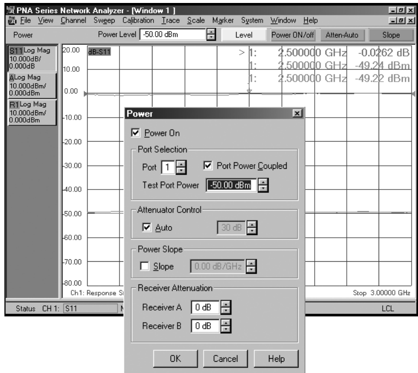
Figure 3. Case B, -50 dBm power level, 30 dB source attenuator
