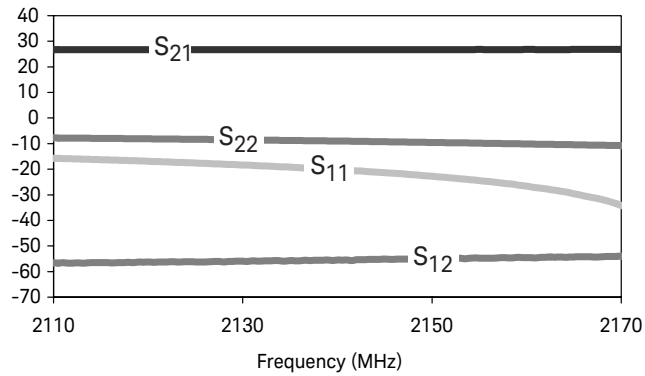
Figure 7. S-parameters of high-power amplifier, under low-power (linear) conditions
