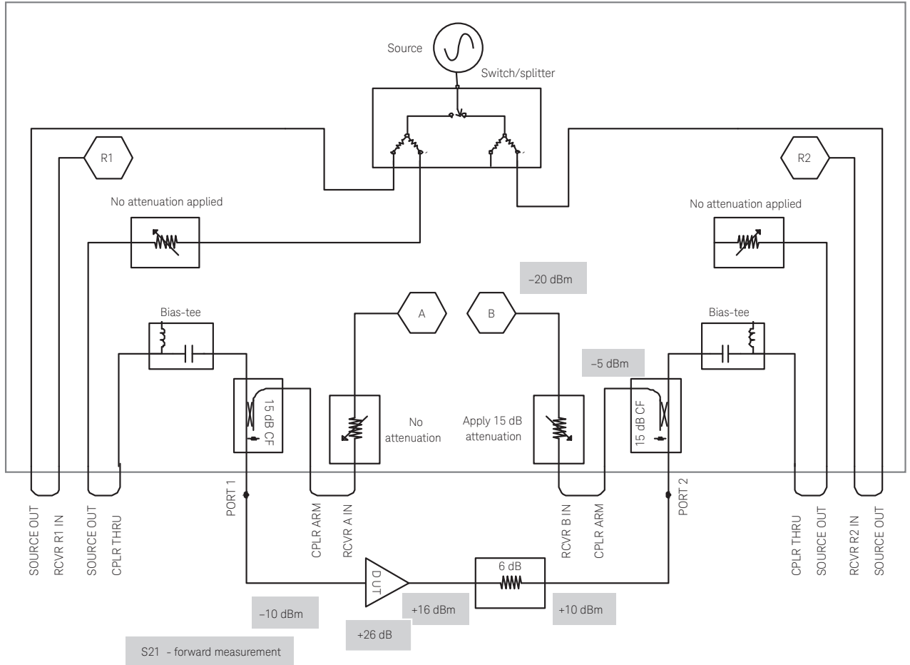
Figure 5. MW PNA E8364B for testing handset amplifier – low input power
