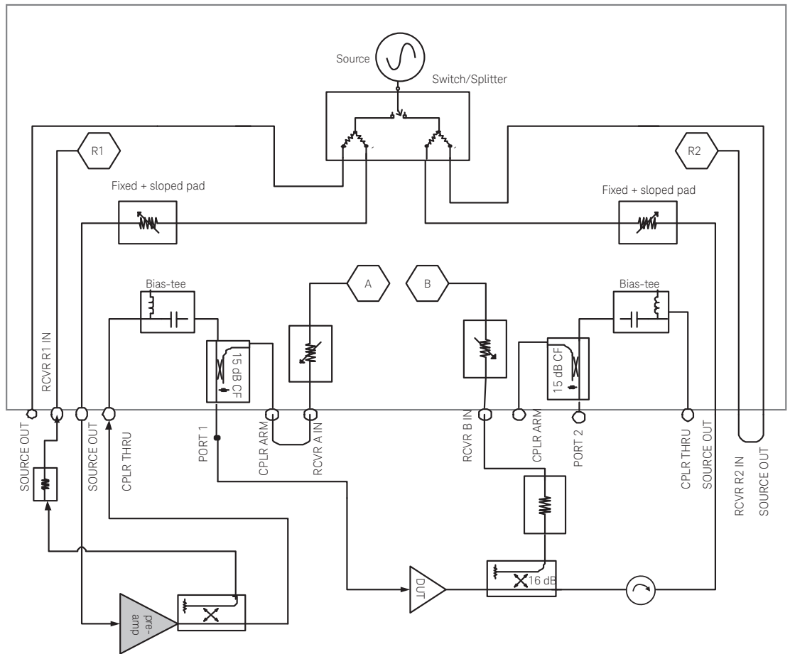
Figure 13. Use of external coupler in high-power measurements
