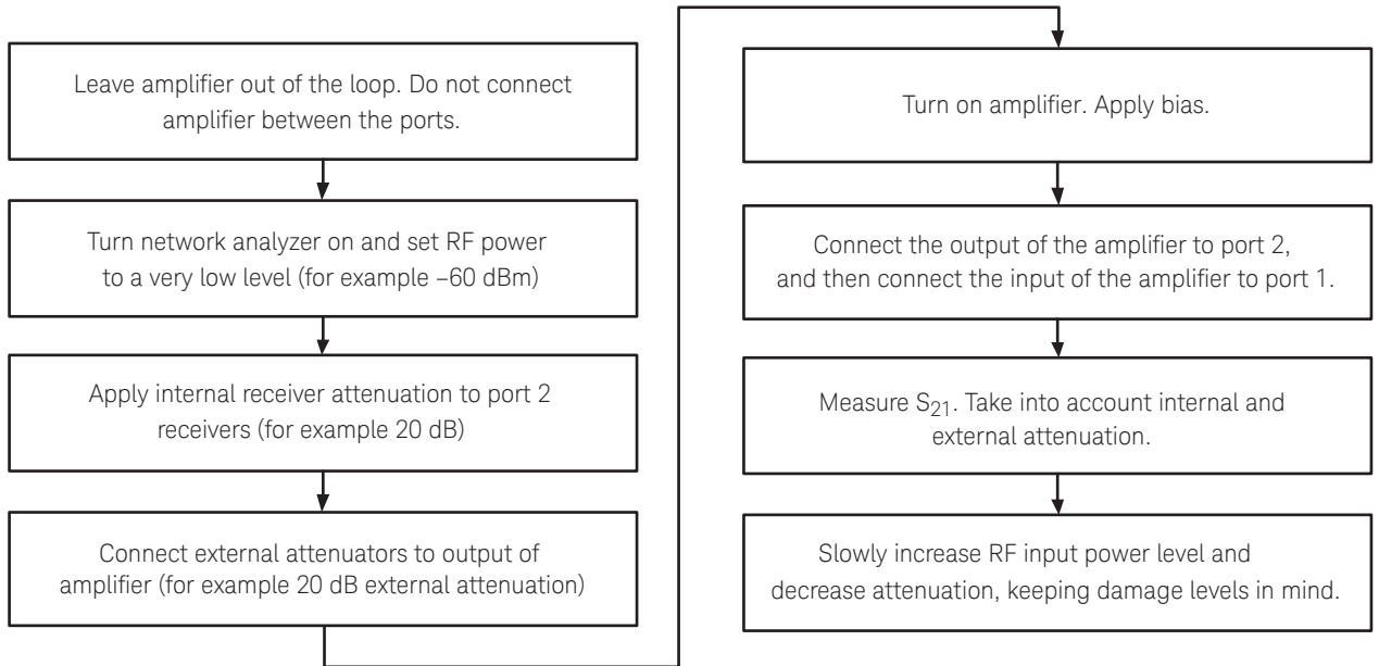
Figure 6. Procedure and sequence to connect amplifier to network analyzer
