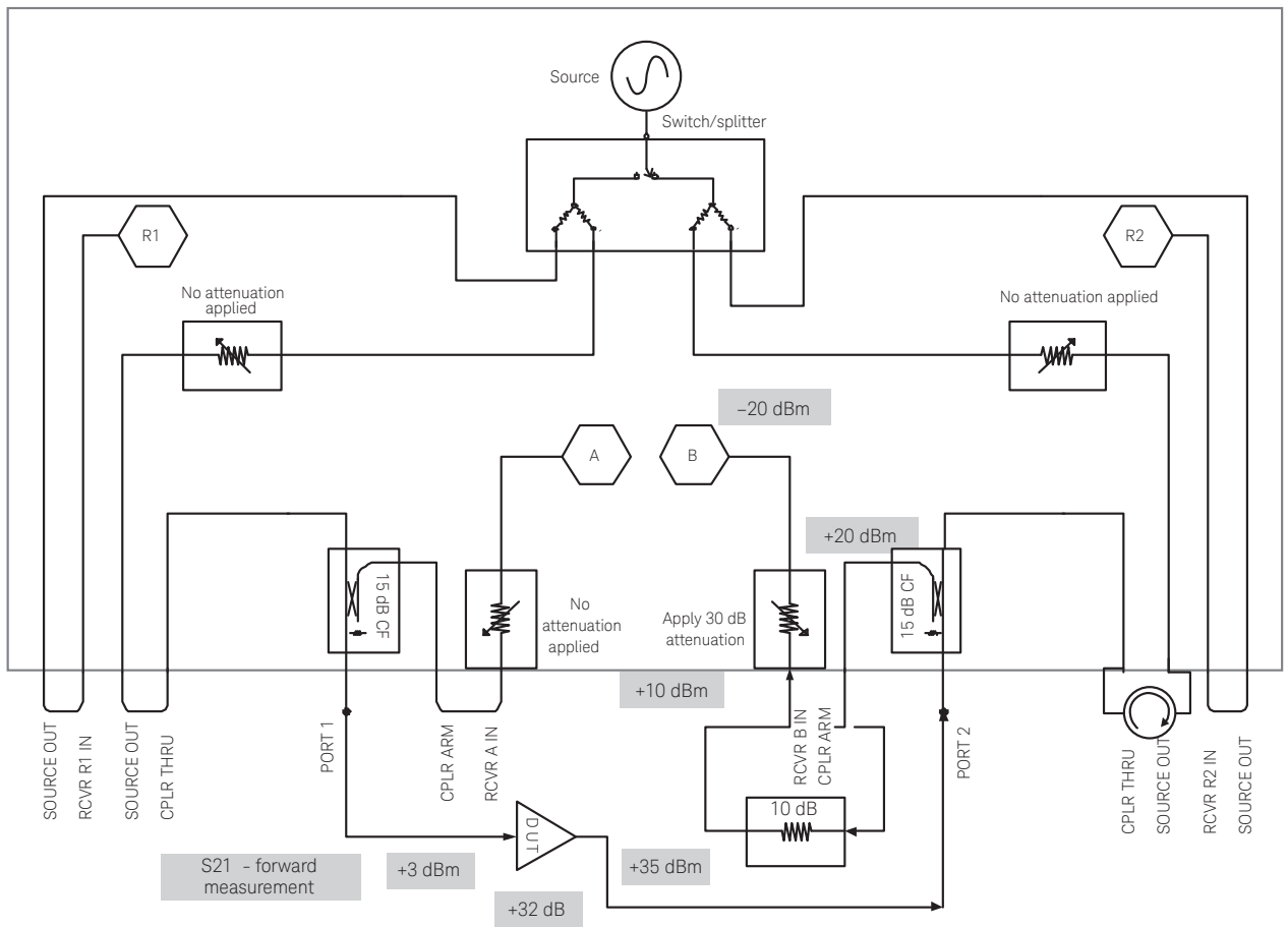
Figure 3. MW PNA E8362B-H85, configured to measure a dual band handset amplifier
