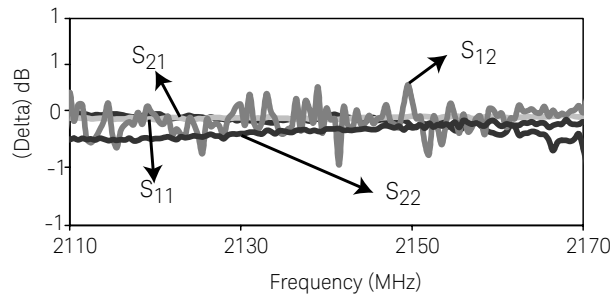
Figure 10. Difference in S-parameters, when tested with and without pre-amplifier
