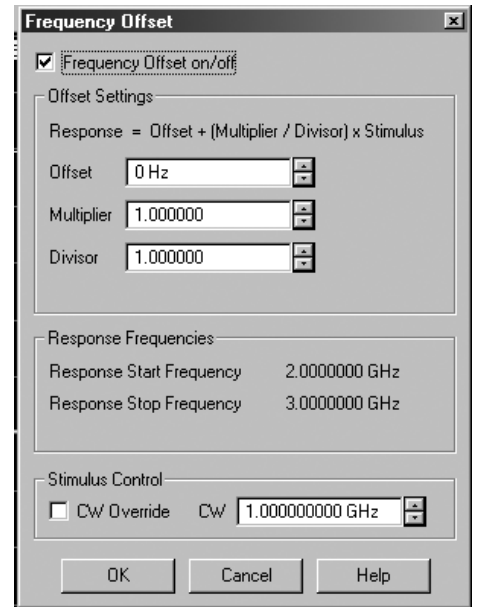
Figure 6. Use frequency-offset mode to take advantage of independent phase-locking circuitry
