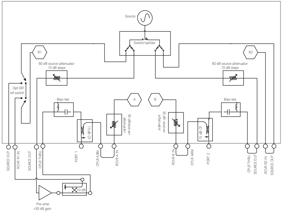
Figure 4. High-power setup connection diagram
