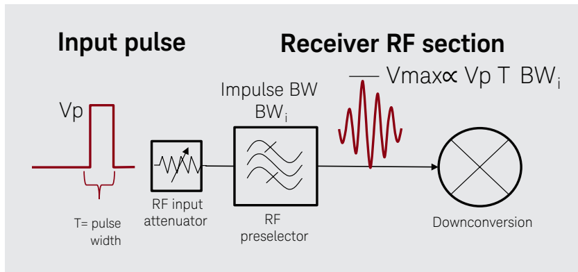
Figure 3. Preselector impulse bandwidth limits impulse input voltage to receiver downconversion chain
