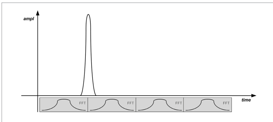
Figure 2a. Traditional critically-sampled FFTs with contiguous windows has potential for missing input impulsive signal
