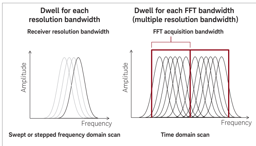
Figure 1. Comparison of resolution and FFT acquisition bandwidths
