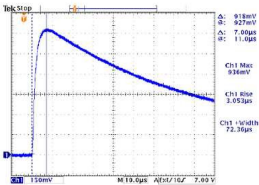
WF1 Iron core (300A current)
