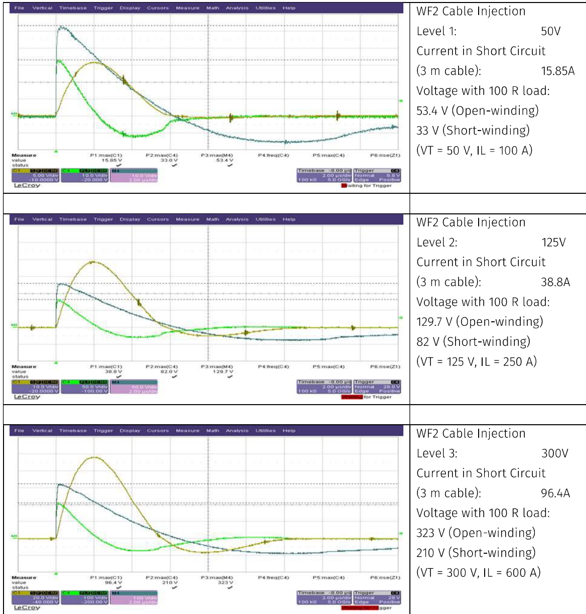
Figure 5: Voltage across 100Ω (WF2) and current in short circuit (WF1).
