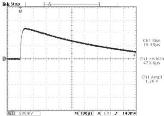
WF5B Iron core not saturated
