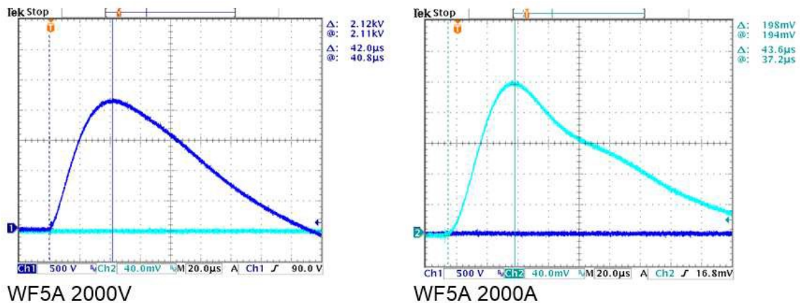
Figure 7: Hybrid coupler waveform open and short circuit for WF5A.
