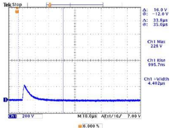
WF1 Iron core (voltage @ 300A)
