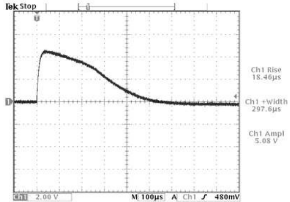
WF5B Iron core in saturation
