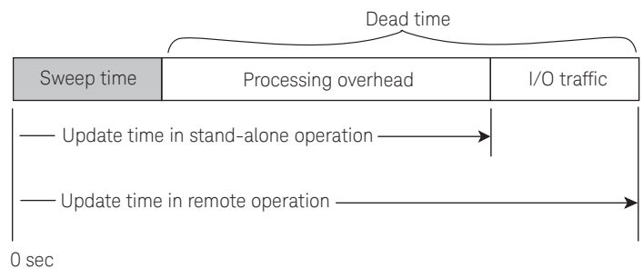
Figure 1. The components of measurement update time.
