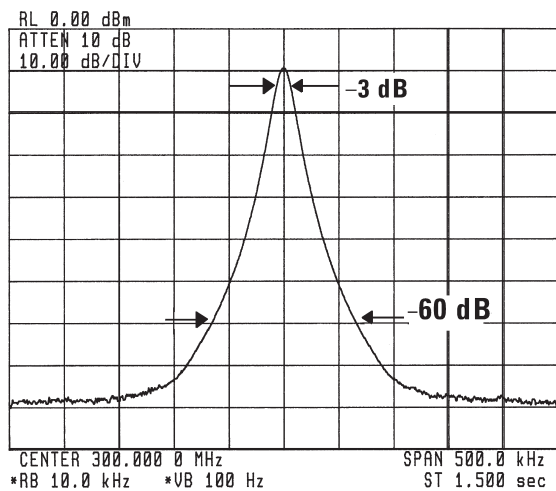
Figure 2. RBW selectivity is the ratio of the width at -60 dB to the width at -3 dB.
