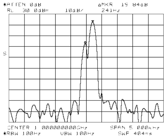
Figure 6. 100 Hz digital RBW filter
