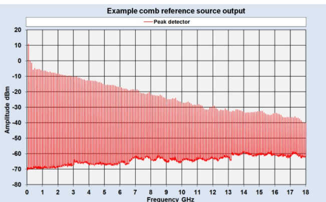
Figure 6: Example comb reference source output
