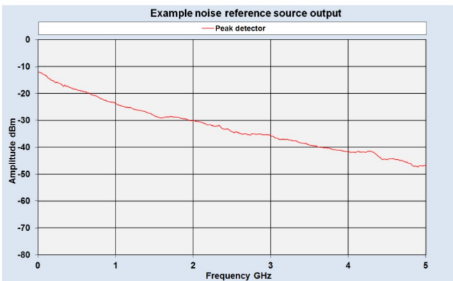
Figure 5: Example noise reference source output
