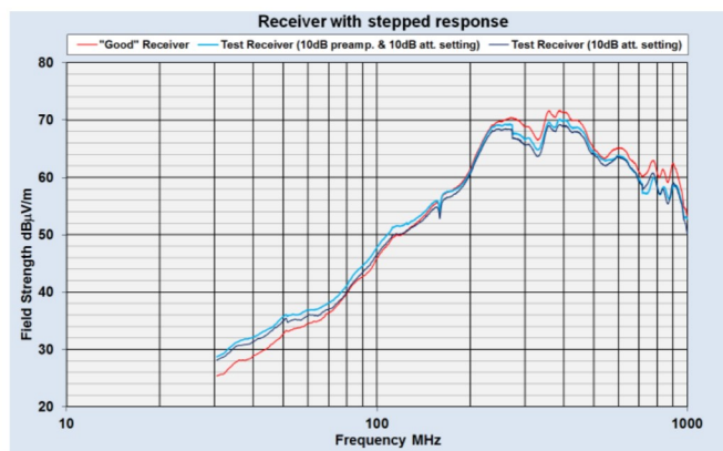
Figure 4: Example of an anomalous receiver response
