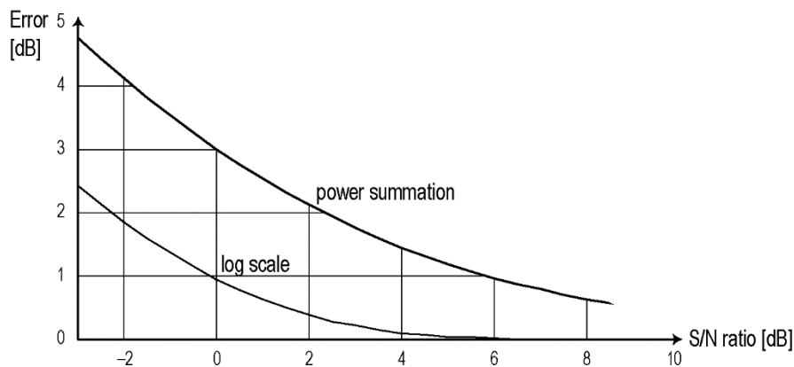
Figure 20. CW signals measured on a logarithmic scale show very little effect due to the addition of noise signals
