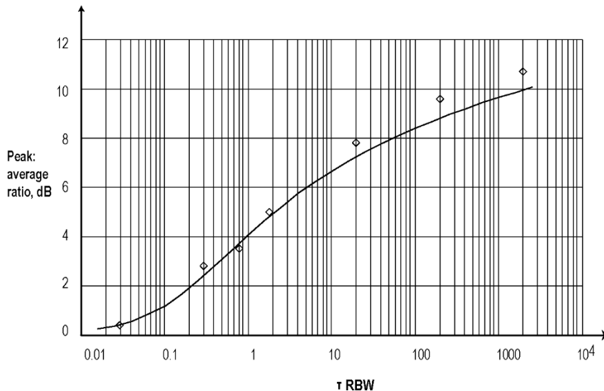
Figure 14. The peak-detected response to noise increases with the observation time
