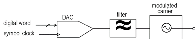
Figure 12. A simplified model for the generation of digital communications signals
