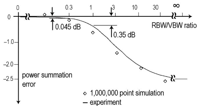
Figure 13. For VBW \geq 3 RBW , the averaging effect of the VBW filter does not significantly affect power-detection accuracy.
