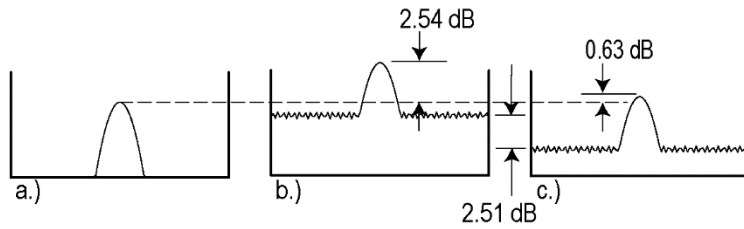
Figure 18. Log averaging improves the measurement of CW signals when their amplitude is near that of the noise. (a) shows a noise-free signal. (b) shows an averaged trace with power-scale averaging and noise power 1 dB below signal power; the noise-induced error is 2.5 dB. (c) shows the effect with log-scale averaging—the noise falls 2.5 dB and the noise-induced error falls to only 0.6 dB.
